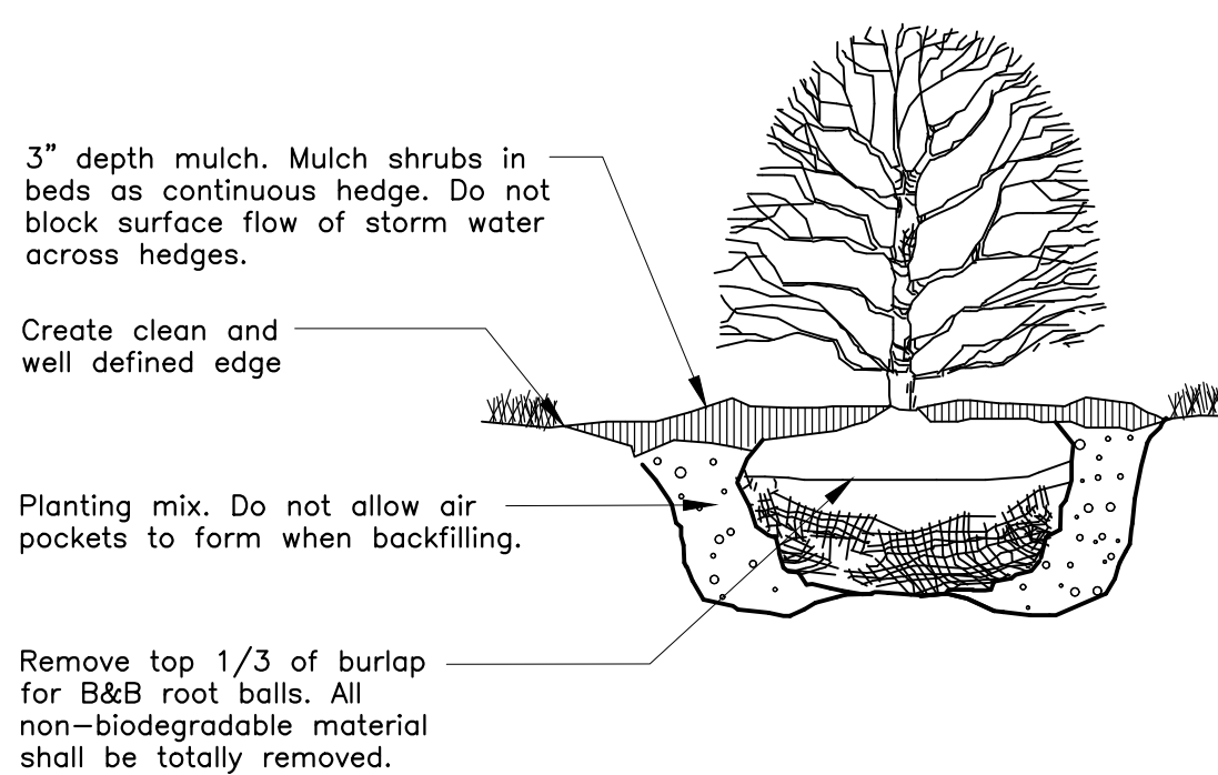
Shrub Planting Not to Scale
