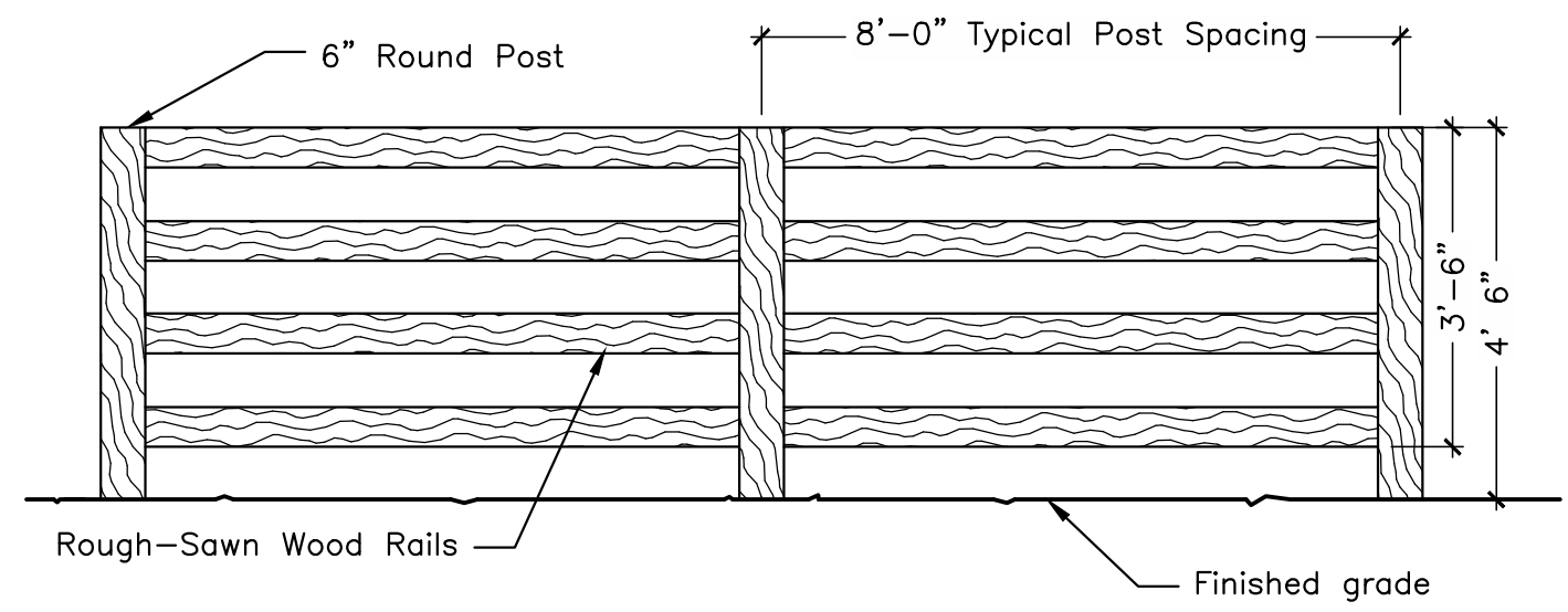
4 Rail Fence Elevation Not to Scale
